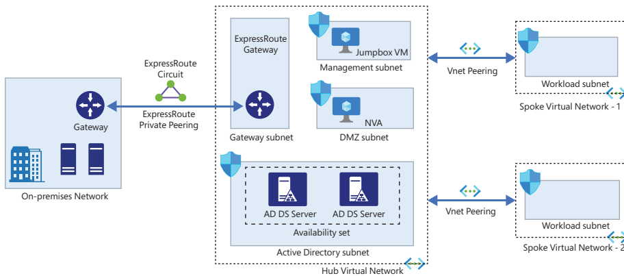
FIGURE 4-7 Hub-and-spoke topology
