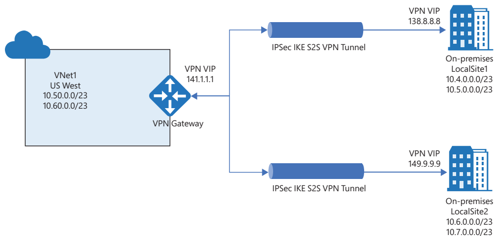
FIGURE 4-13 VPN Gateway
