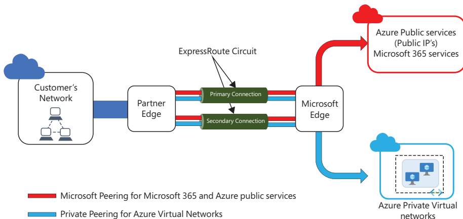
FIGURE 4-12 ExpressRoute
