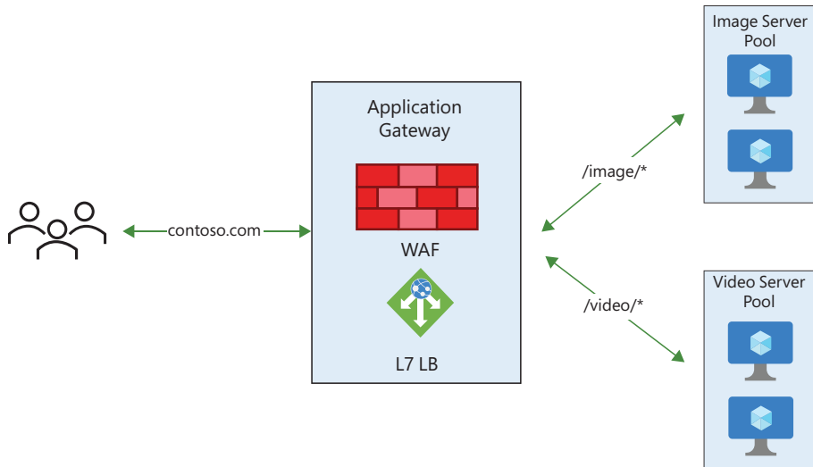
FIGURE 4-17 Application Gateway
